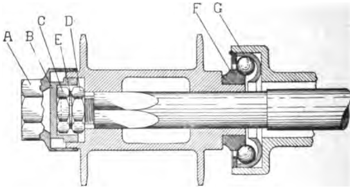
FIG. 460.—One Form of Driving Axle Using Ball Bearings. The hub is secured in place by the nuts and binders shown at A, B, C, D, E. At its inner extremity it carries a cone, F, which works on the ball race, G. The hub is thus suspended on the ball race, which also acts to neutralize end thrusts.
